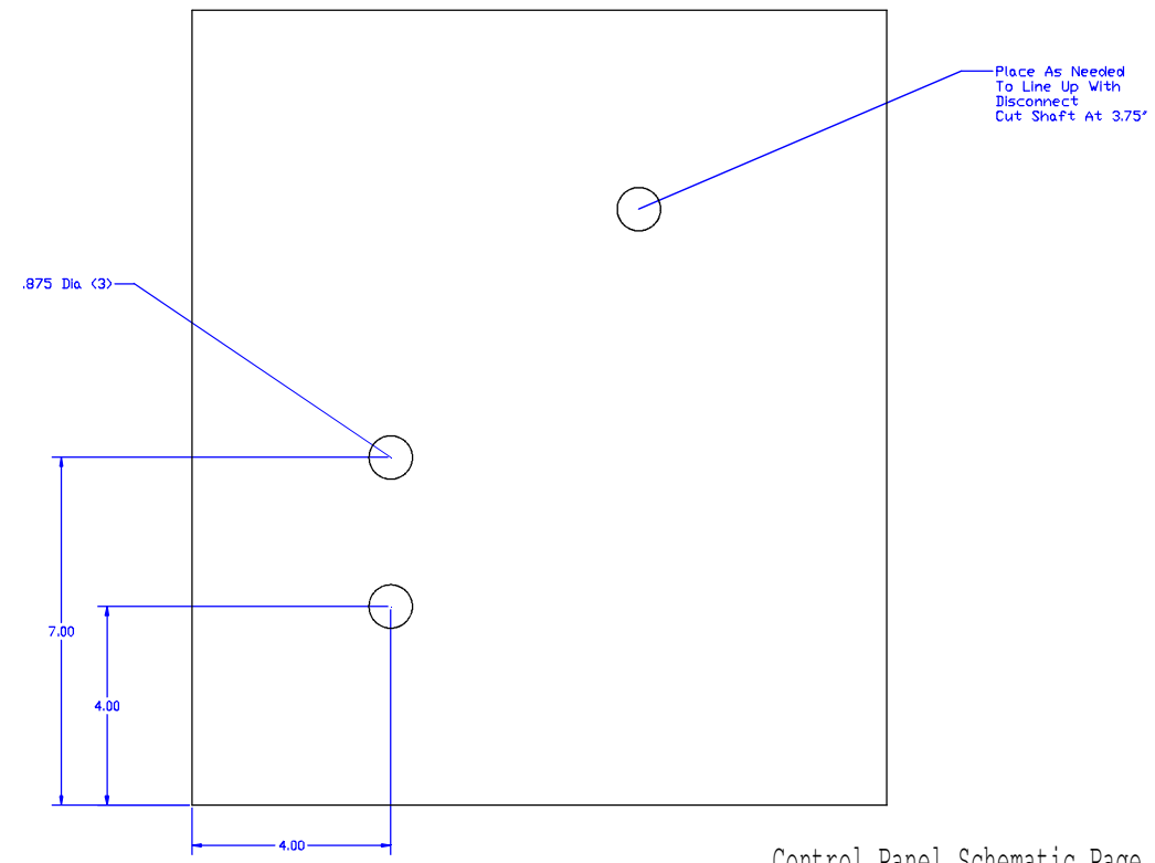
Control Panel Schematic Page 1 of 1
